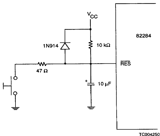
Figure 2. Typical RC RES Timing Circuit
