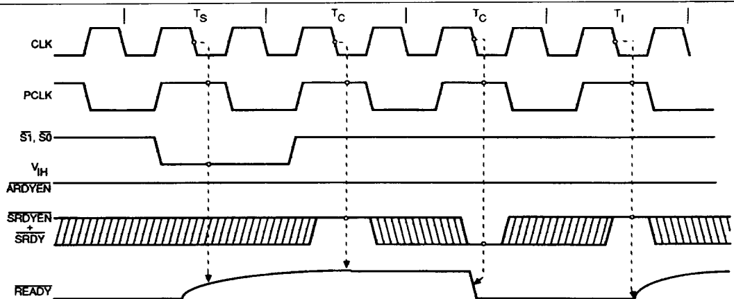
Figure 3. Synchronous Ready Operation
