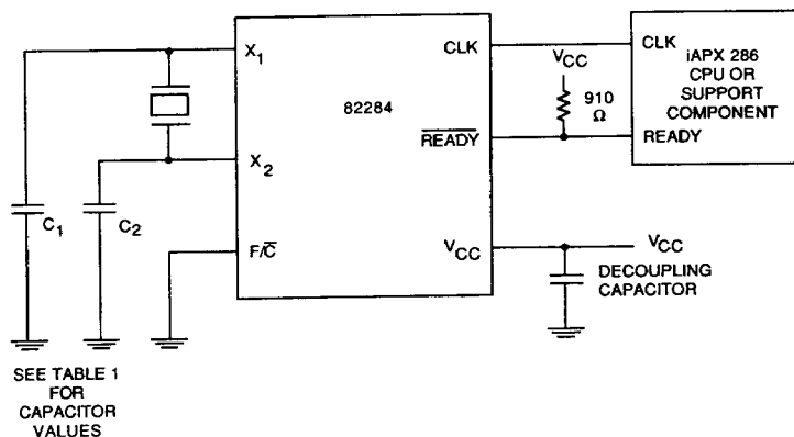
Figure 1. Recommended Crystal and READY Connections
